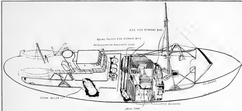
FIGURE 1 - CUTAWY VIEW OF THE DELAWARE , SHOWING LOCATION OF THE REFRIGERATION SYSTEM AND STORAGE BINS.
